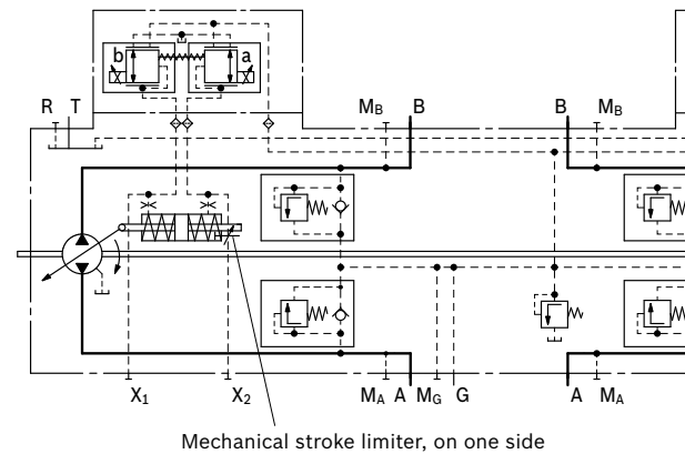
Mechanical stroke limiter, on one side
