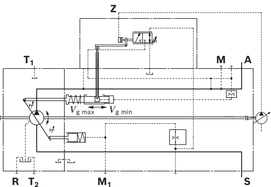
▼ Circuit diagram NG 190 to 260
