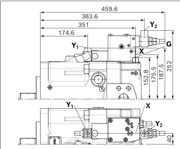
▼ LG1GH2 – Power controller, pilot-pressure related override
