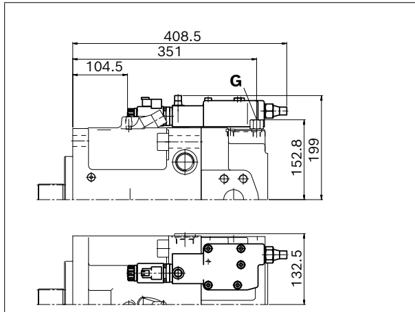
▼ DRS/DRG – Remote-controlled pressure controller, load sensing
