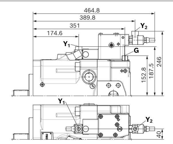
▼ LG2H2 – Power controller, pilot-pressure related override
