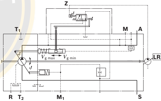
▼ Circuit diagram NG 190 to 260
