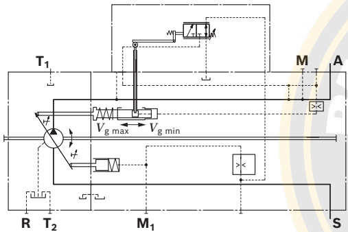
▼ Circuit diagram NG 190 to 260
