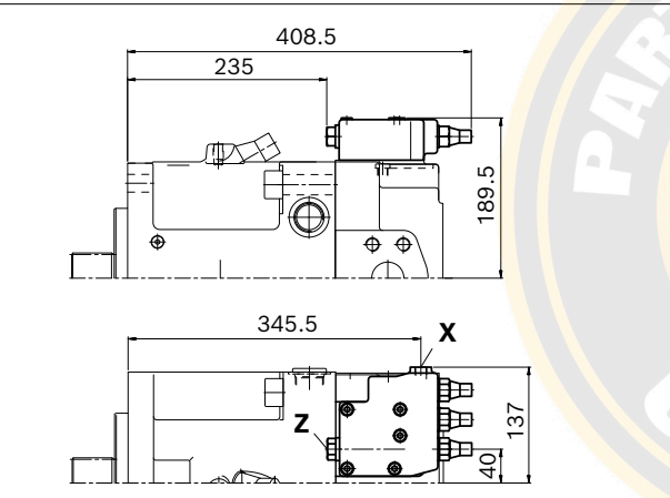
▼ LG2H2 – Power controller, pilot-pressure related override
