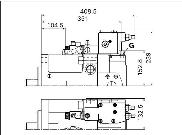
▼ LG1GH2 – Power controller, pilot-pressure related override
