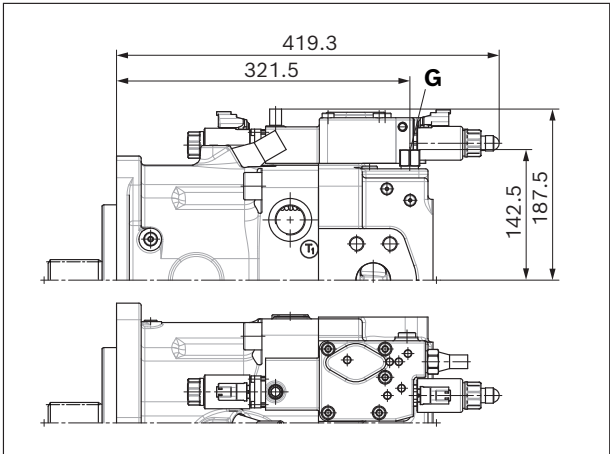
▼ DRL – Pressure controller, parallel operation
