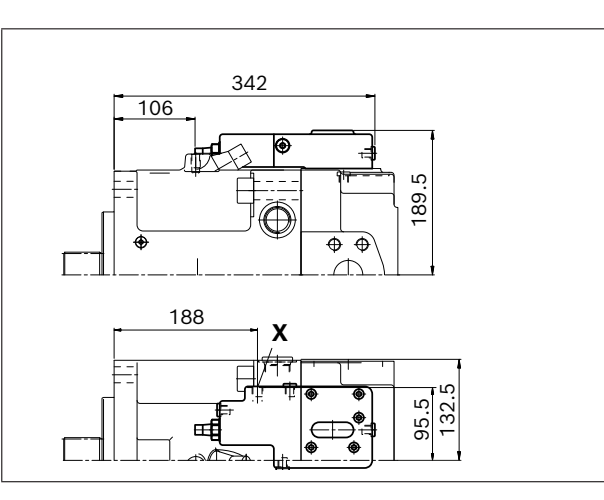
▼ DRL – Pressure controller, parallel operation
