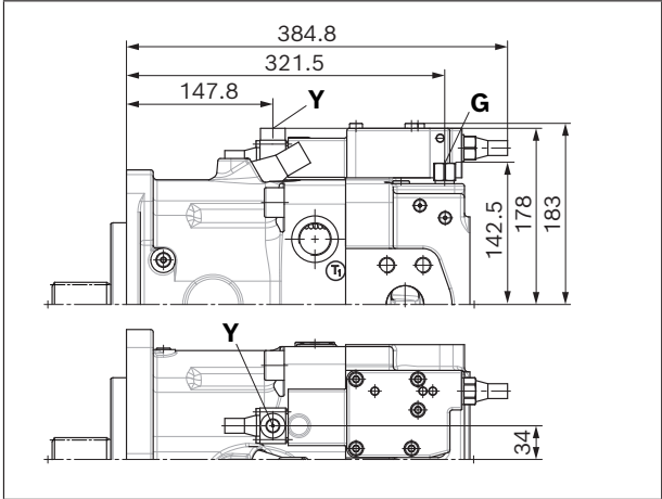
▼ EP2G2 – Electric control with electrically overridable pressure cut-off (positive control)
