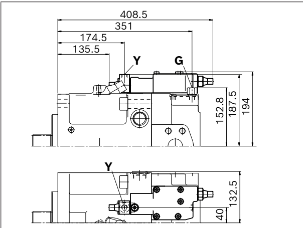
▼ EP2G2/EP2G4 – Electric control with electrically overridable pressure cut-off (positive/negative control)
