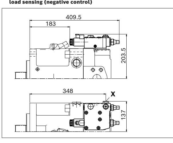
▼ LE2S – Power controller, electrical override, load sensing (negative control)
