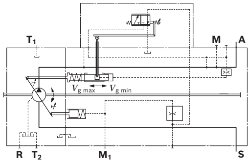
▼ Circuit diagram NG 40 to 145
