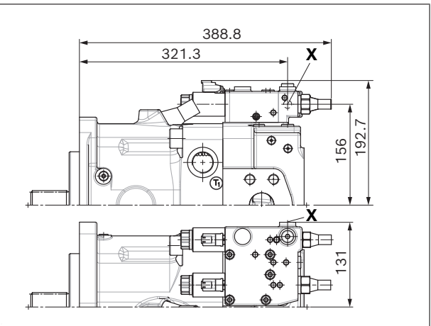
▼ LE2S2/LE2S5 – Power controller, electrical override, load sensing, overridable
