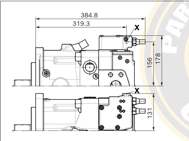
▼ LE2S – Power controller, electrical override, load sensing (negative control)
