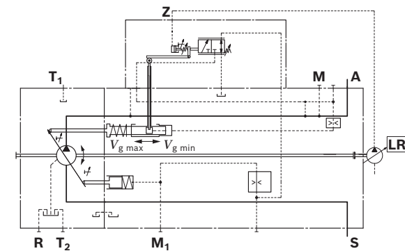
▼ Circuit diagram NG 190 to 260
